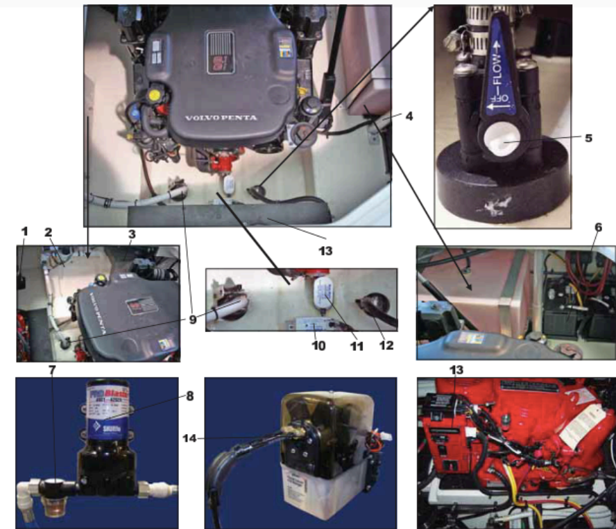
1. GENERATOR MUFFLER 2. VACUFLUSH WASTE TANK 3. HOT WATER HEATER 4. DECK SUPPORT BRACE 5. SEA COCK (SEACOCK SHOWN IN PARALLEL OPEN POSITION) 6. BATTERY TRAYS
